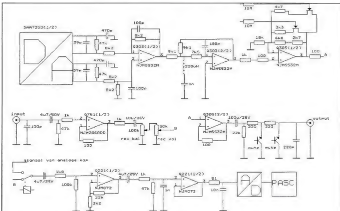
Philips DCC 900
